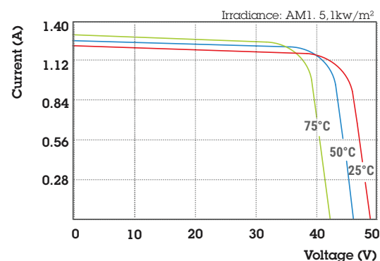
DFE050S-24U I-V Curves
