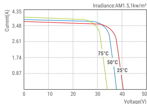
DFE120S-24U I-V Curves
