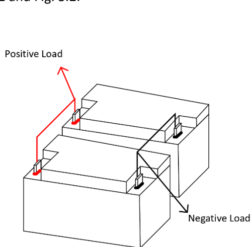
Figure 3.1: Two 1250 Batteries connected in Parallel to create a 12V 100Ah Battery Bank
